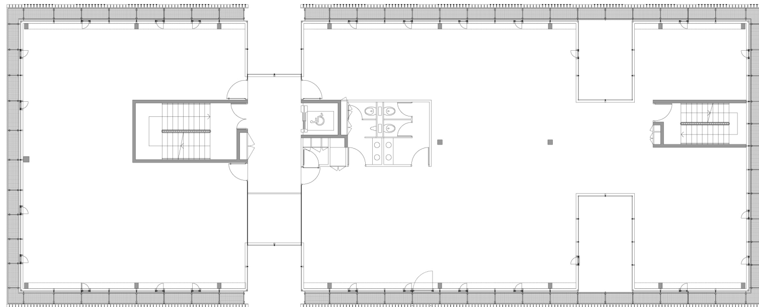
STANDARD FLOOR PLAN [ 2 ] 1/200
