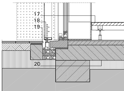
detail 2-4
