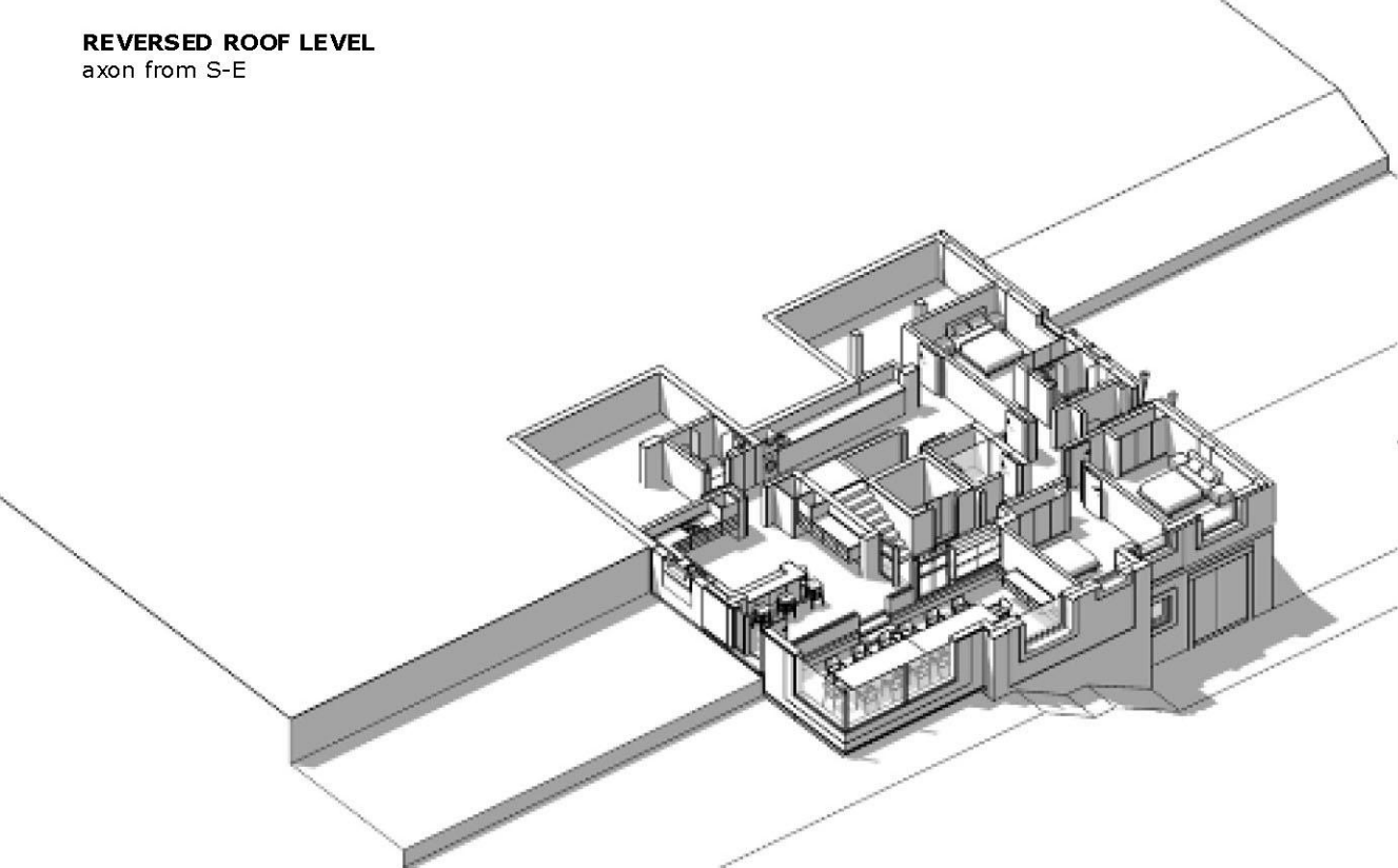
DINING/SLEEPING LEVEL axon from S-E
