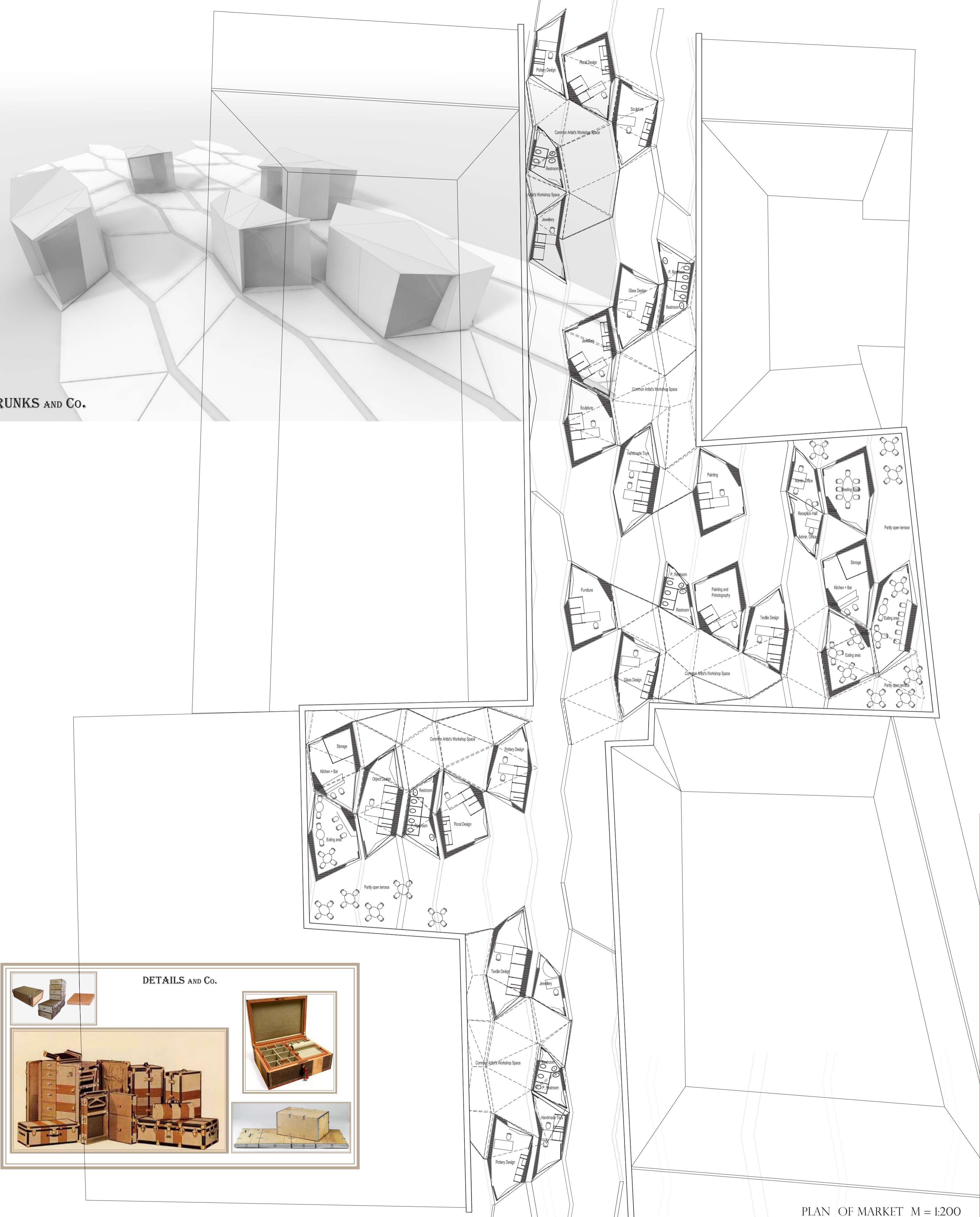
PLAN OF MARKET M = 1:200
