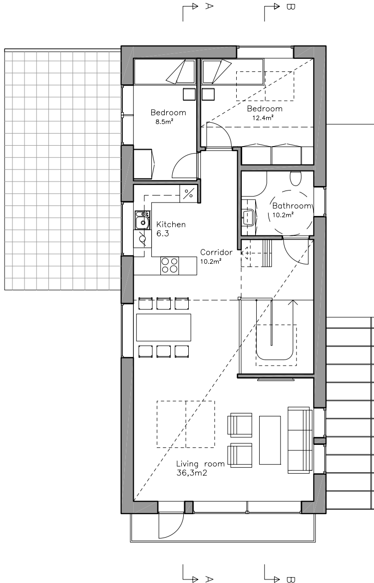
Attic floor
