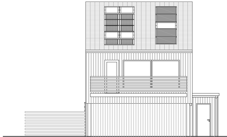
South Facade
