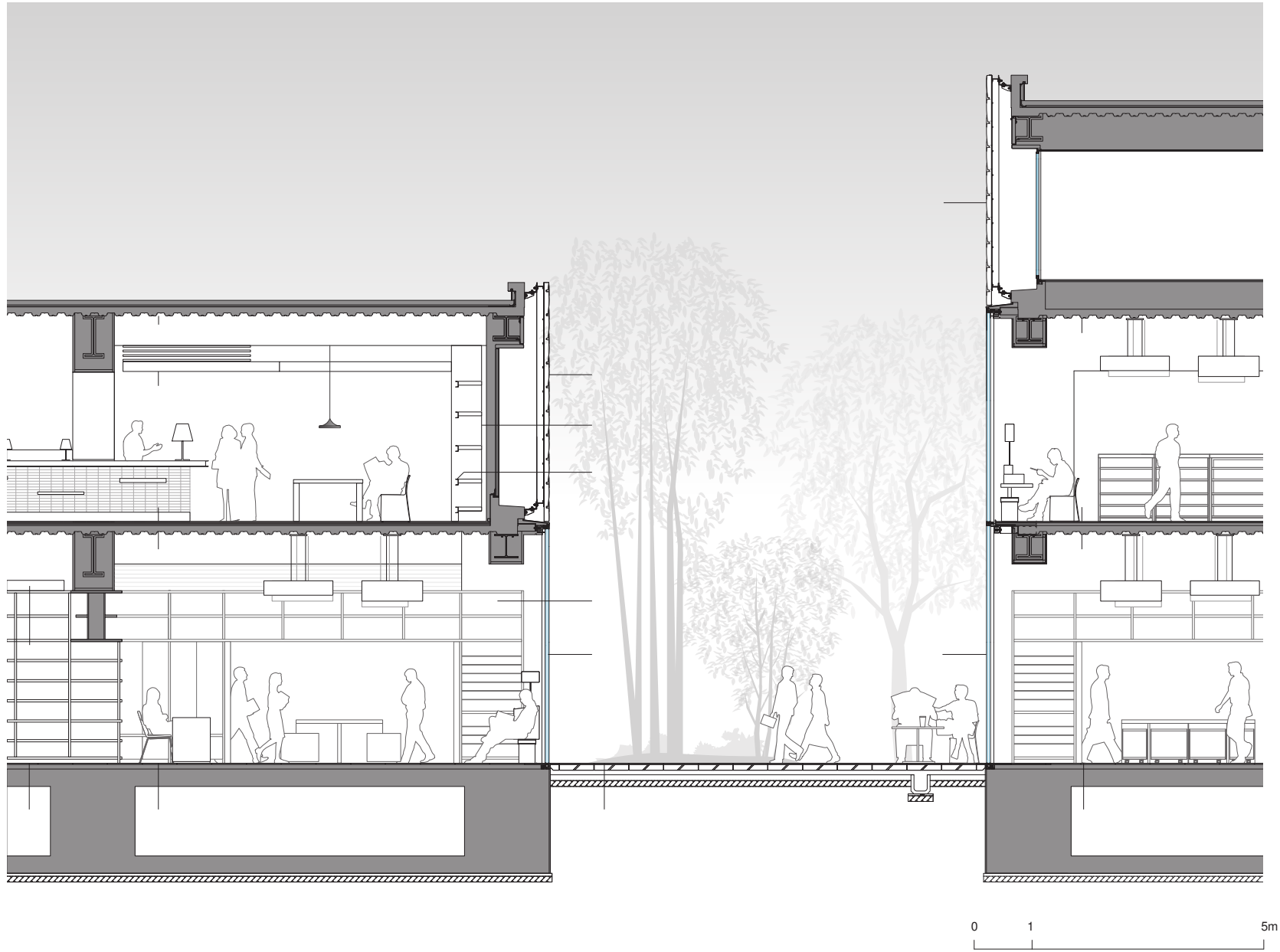
DAIKANYAMA TSUTAYA SECTION S=1:100
