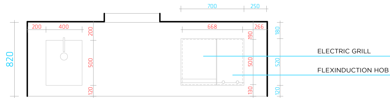
2 SUMMER KITCHEN PLAN IN-402 SCALE 1:25
