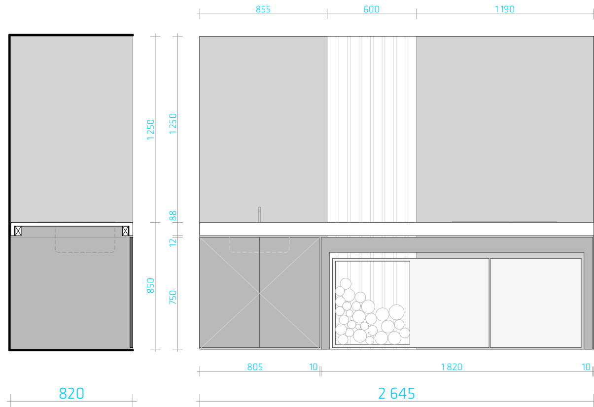
3 SUMMER KITCHEN SECTION IN-402 SCALE 1:25
