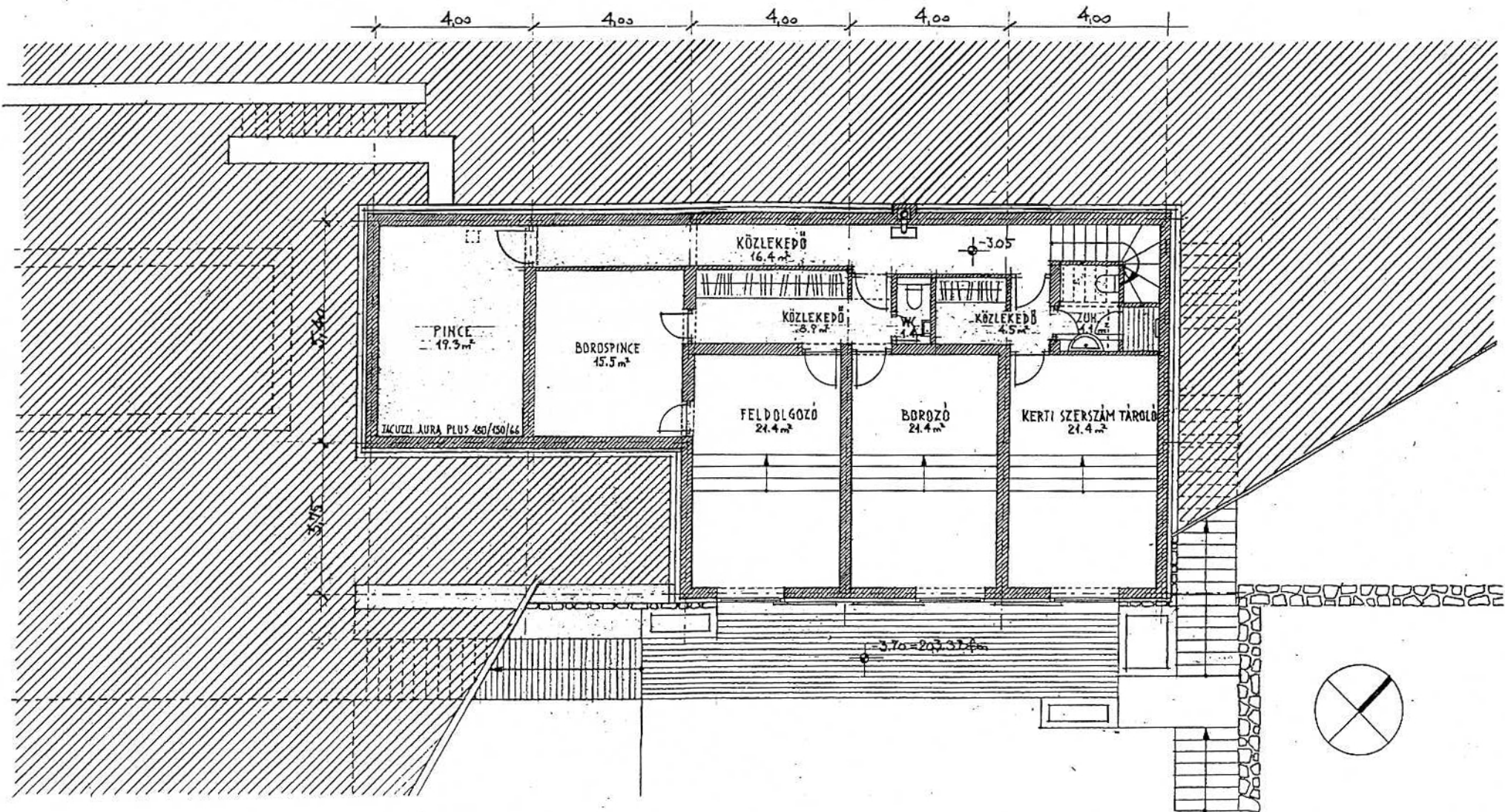
ALSO SZINT ALAPRAJZA - 10. M = 1:100
