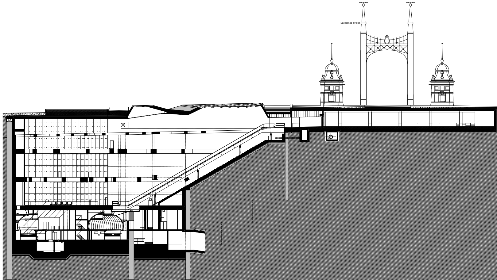
section C-C
