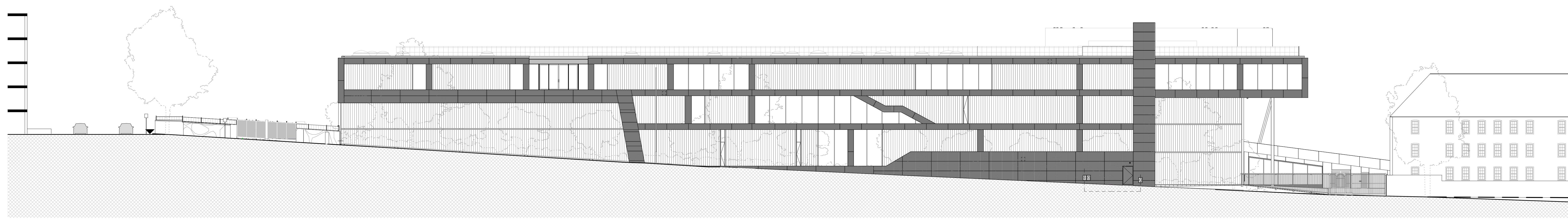
② 06 WEST ELEVATION_SUTHERLAND ROAD 1:200
