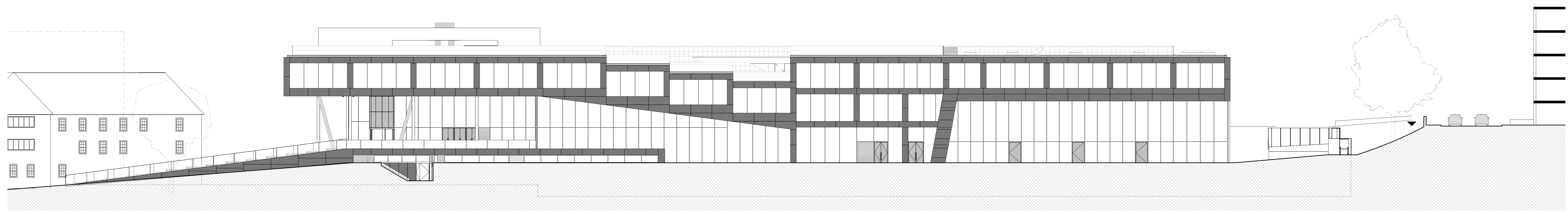
① 06 EAST ELEVATION_FIELD 1:200
