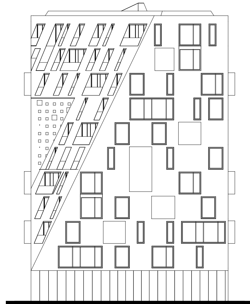
FRONT ELEVATION (x2)
