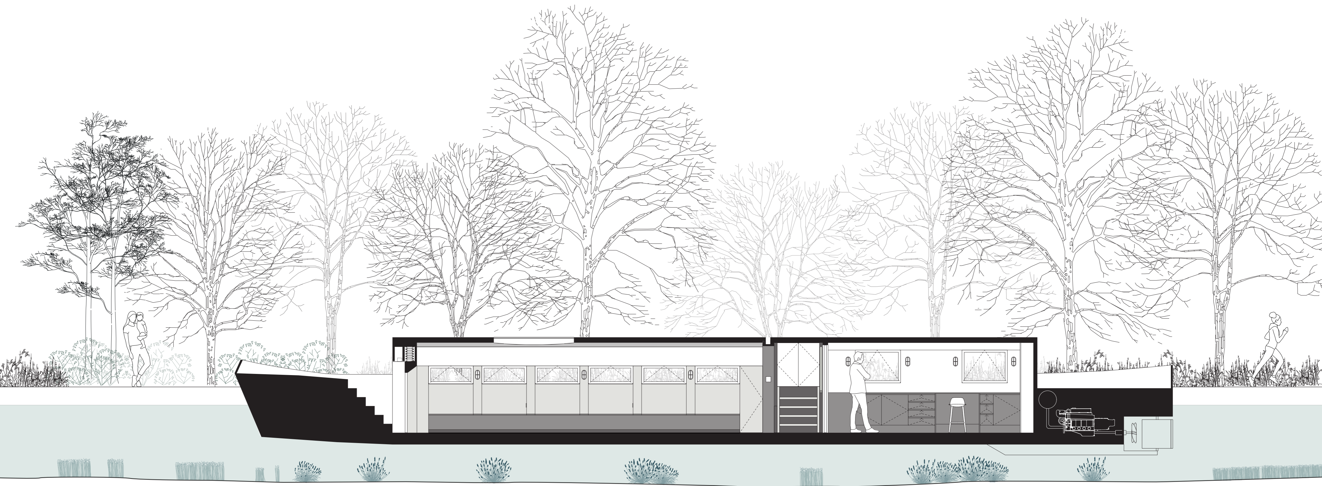
THE FLOATING CHURCH LONG SECTION_ROOF CLOSED 1:25@A2
