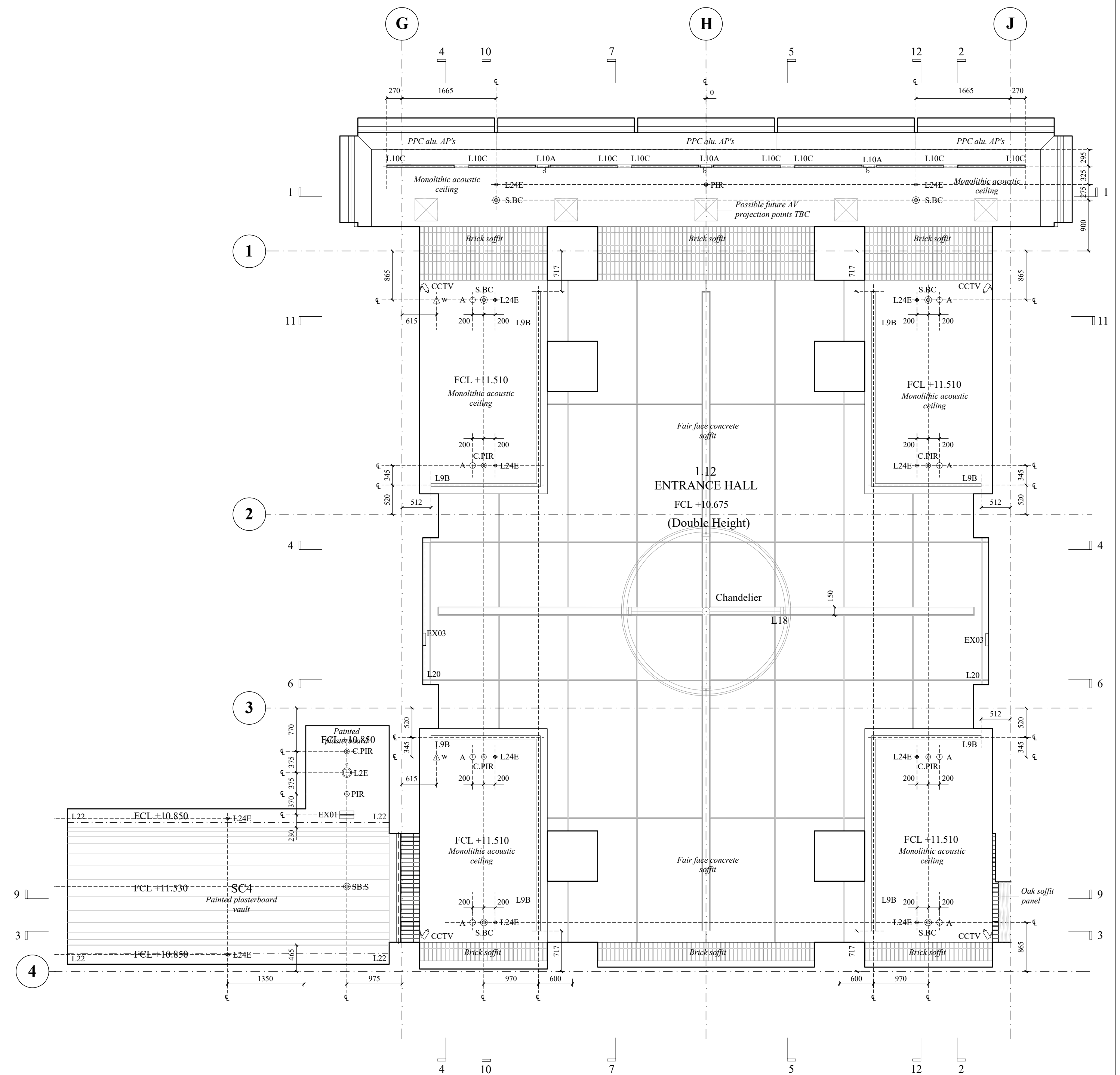
REFLECTED CEILING PLAN
