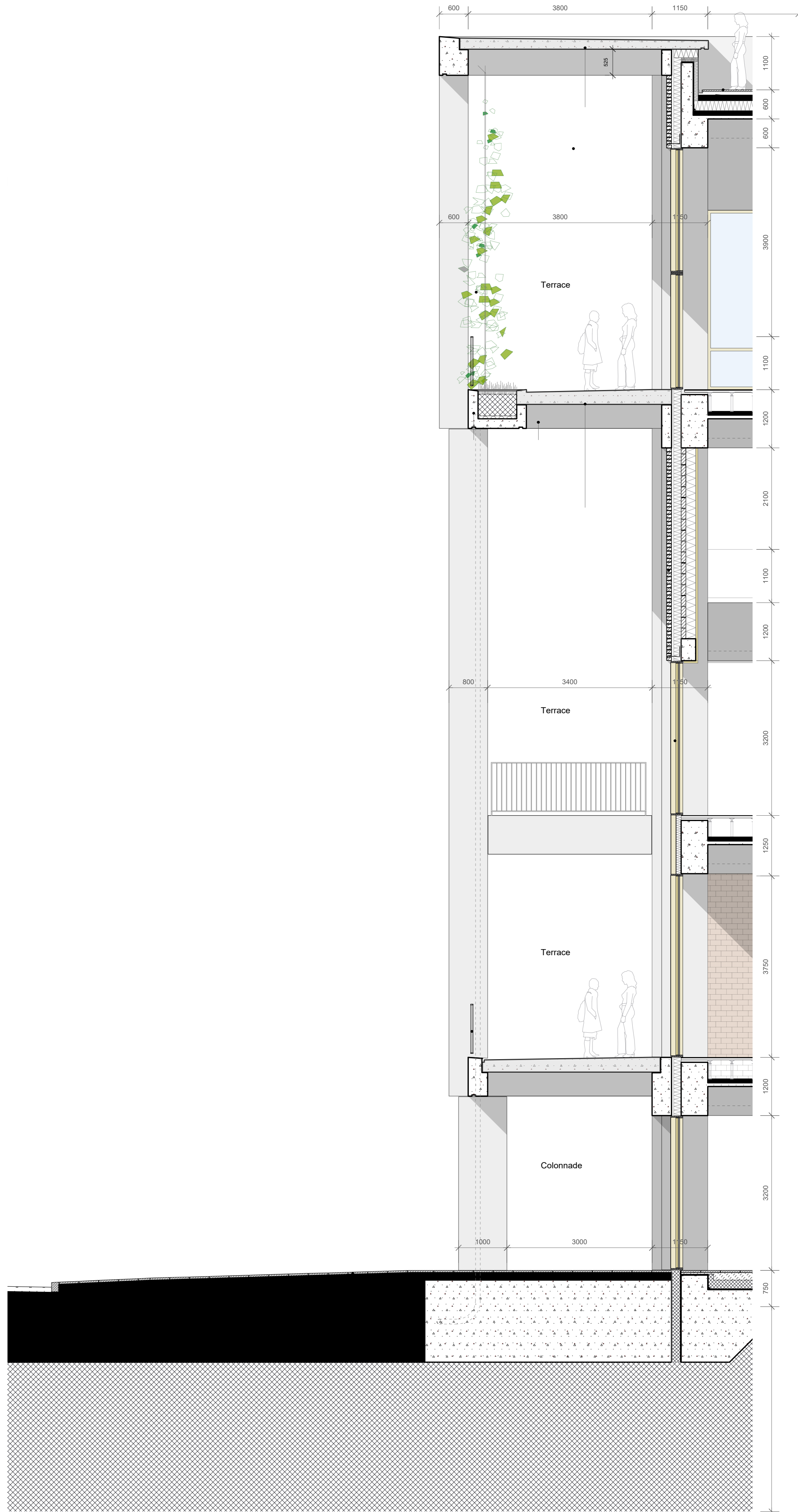
Proposed Facade Detail Section
