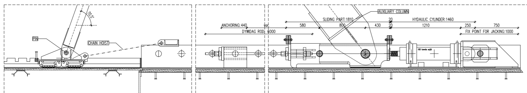
DETAIL R2-R3 AUXILIARY COLUMN - SLIDING MECHANISM - STAGE 1.
