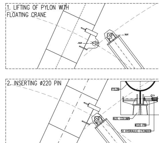
DETAIL R1 PYLON AND AUXILIARY COLUMN CONNECTION
