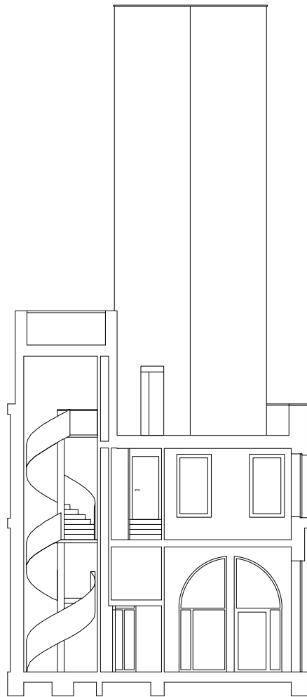
SECTION A
