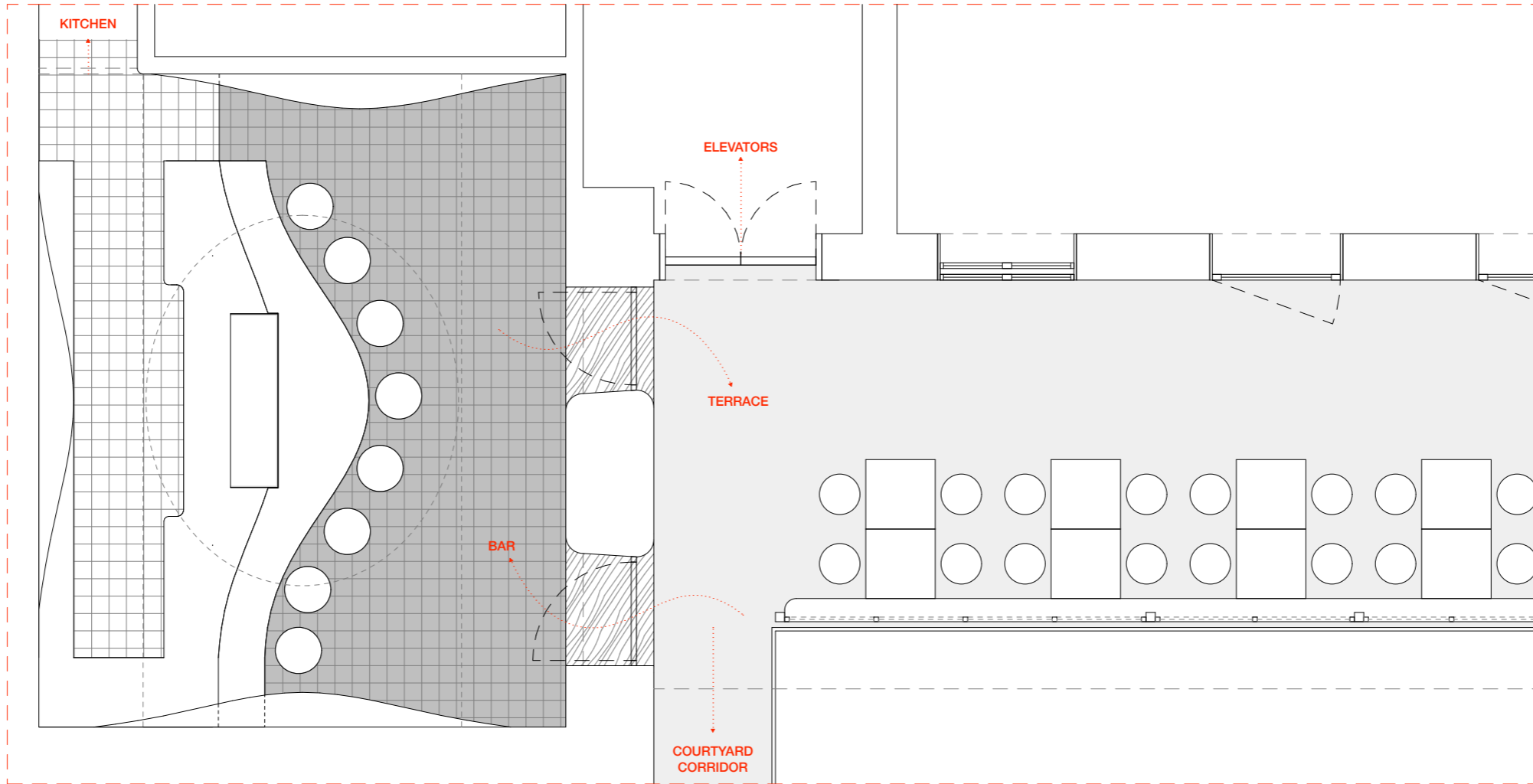
FLOOR PLAN
