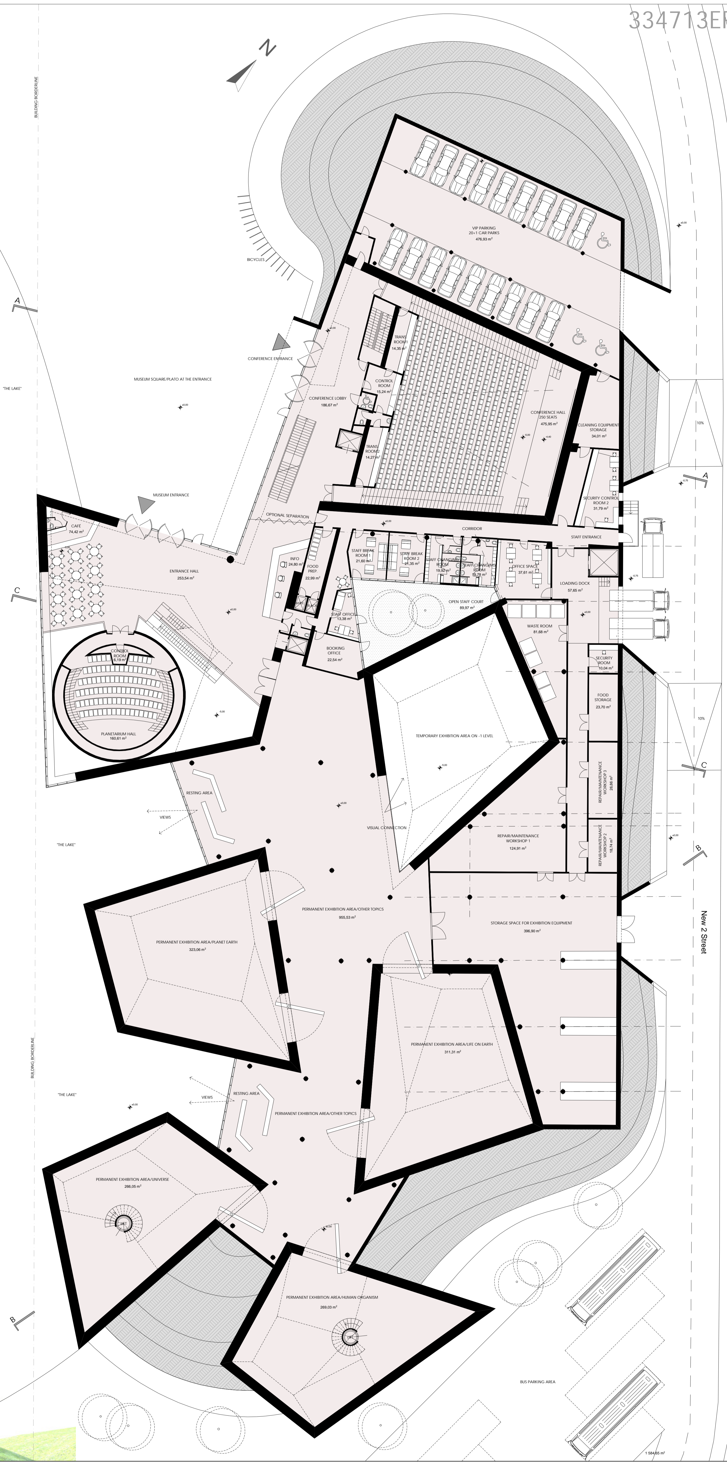
GROUND FLOOR PLAN SCALE-1:200
