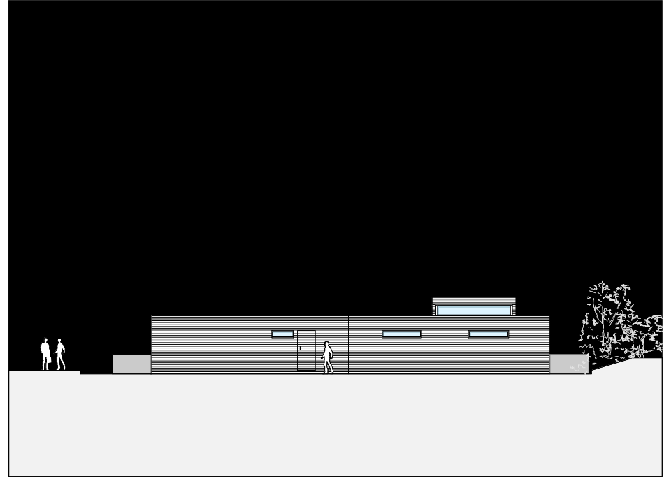
NORTH ELEVATION 1:100
