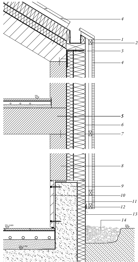
1 - Metal flashing to overhang 25mm over counter batten on wall; 2 - 32x25mm batten; 3 - 38x25mm counter batten / ventilation gap; 4 - Charred cedar fascia board; 5 - Laminated solid wood floor slab; 6 - Vapour permeable membrane; 7 - Wood fibre insulation with water resistant fibre board cover; 8 - Laminated solid wood wall; 9 - Reinforced concrete up-stand as flood defence; 10 - Secret fixed timber board skirting; 11 - Rigid insulation; 12 - 2mm galvanised steel flashing; 13 - Galvanised metal sheet secret fixed; 14 - Flint stone.
