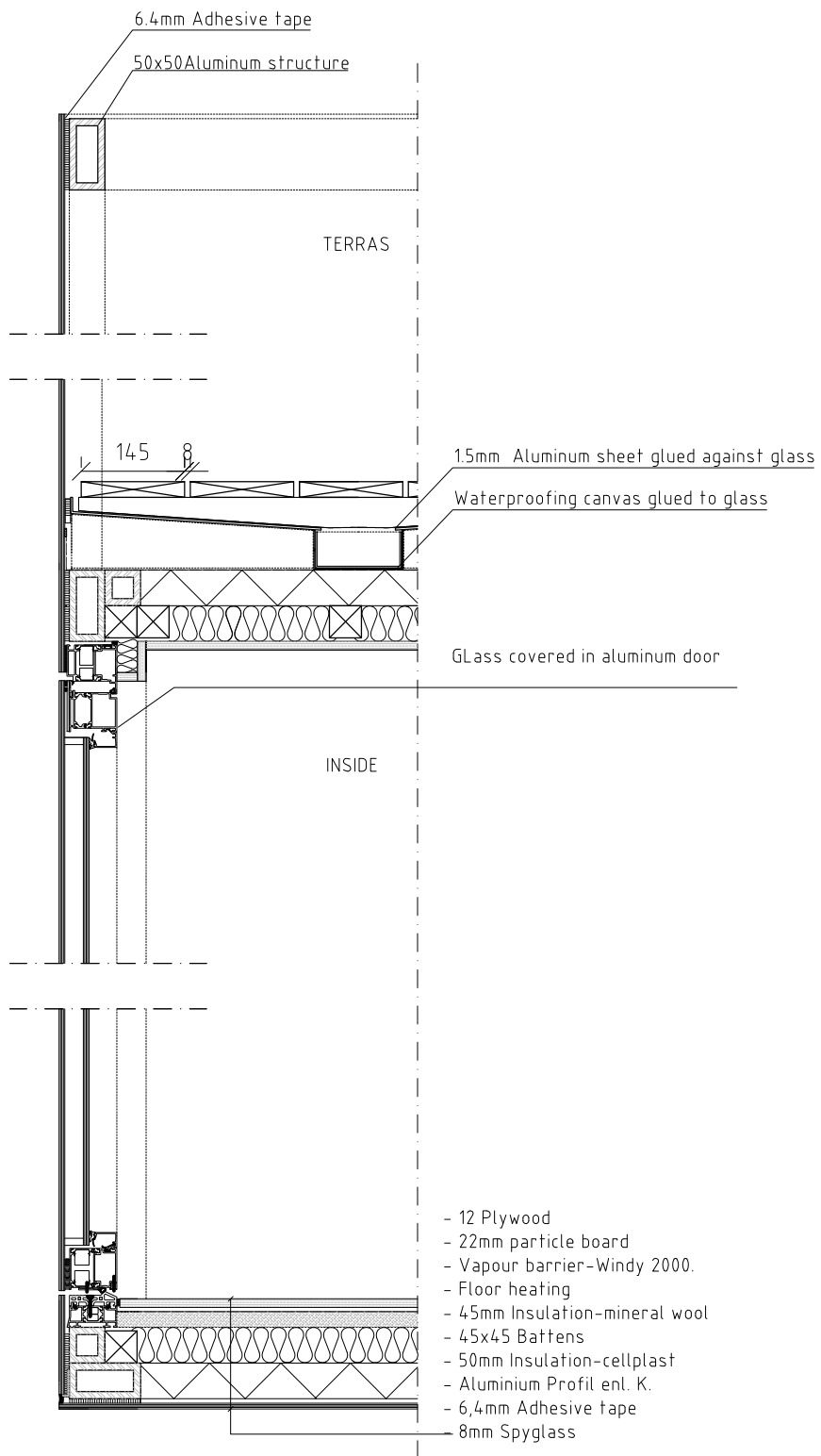
Detail. Vertical section through facade/terras. All measurements in millimetres.
