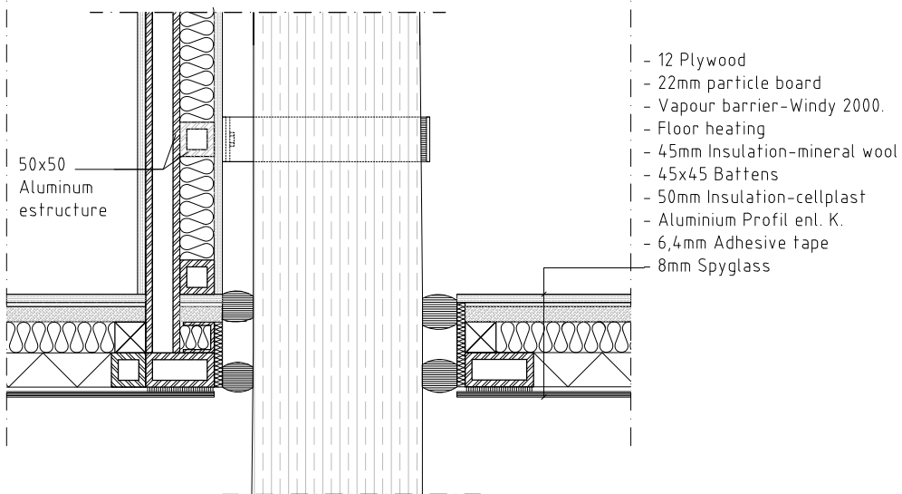
Detail. Vertical section through three measurements in millimetres
