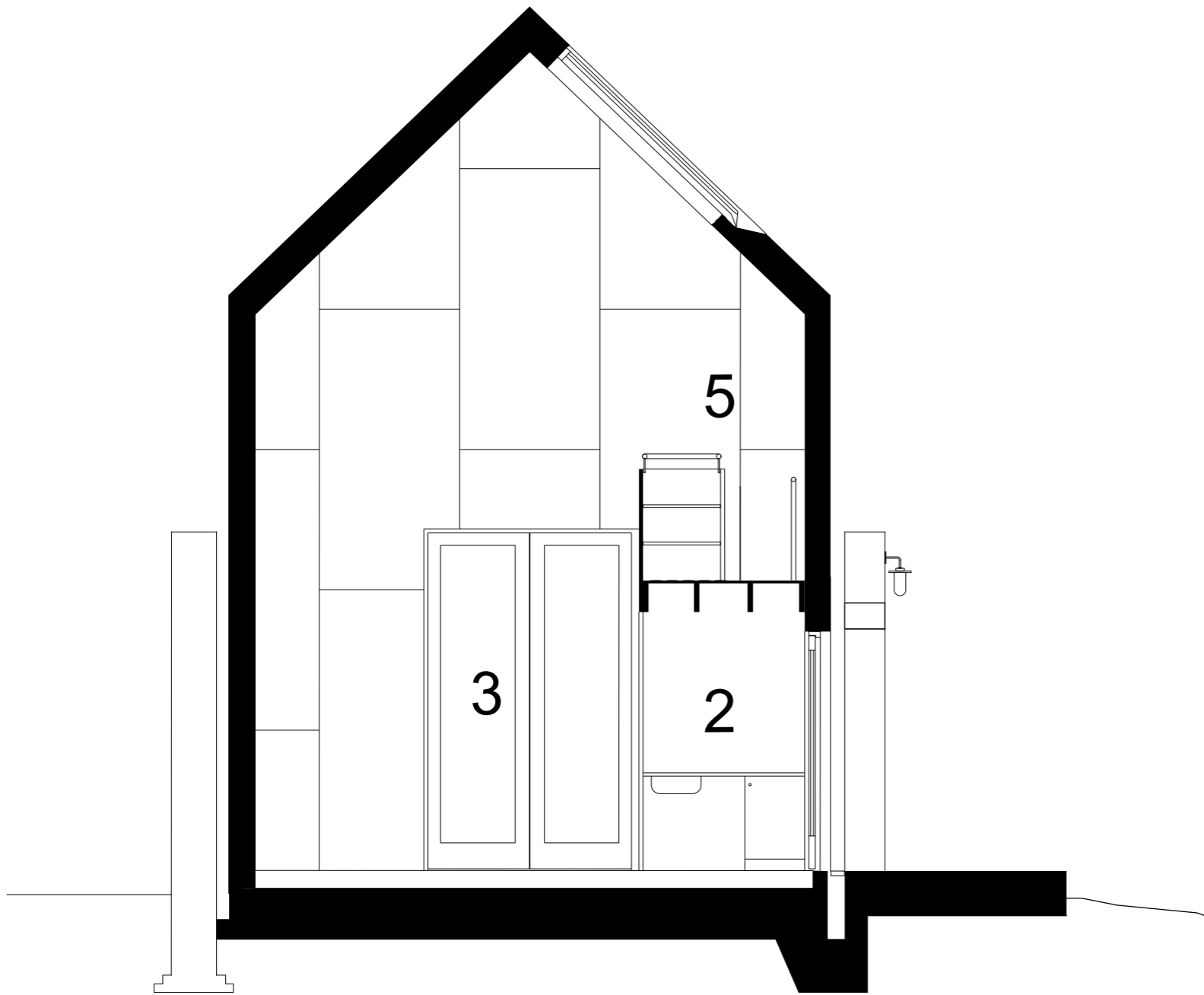
ALDEBURGH MUSIC, DOVECOTE STUDIO SECTION LOOKING WEST
