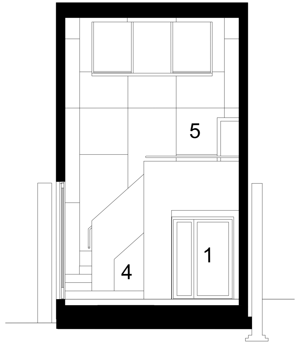
SECTION LOOKING NORTH
