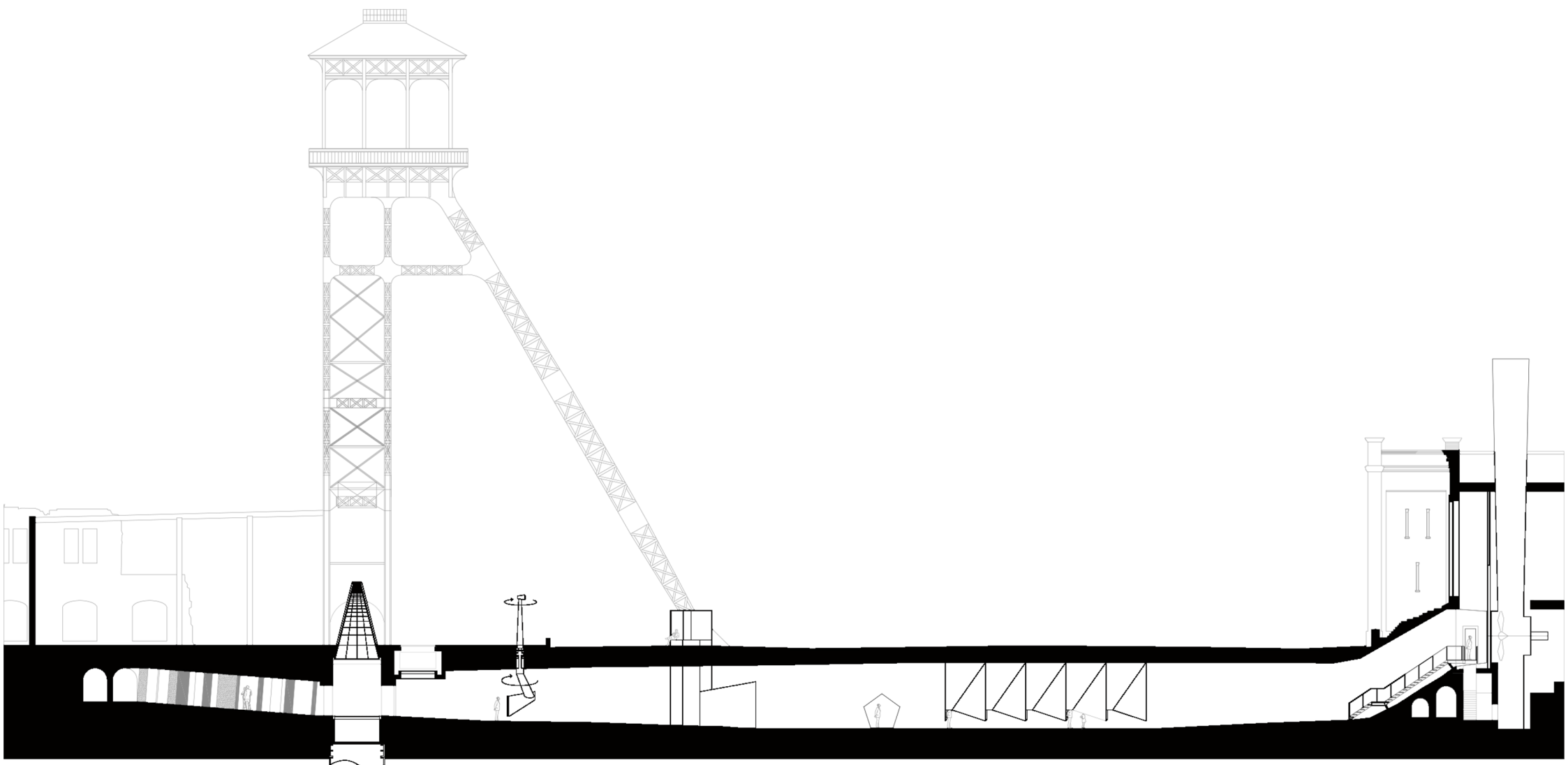
Section BB
