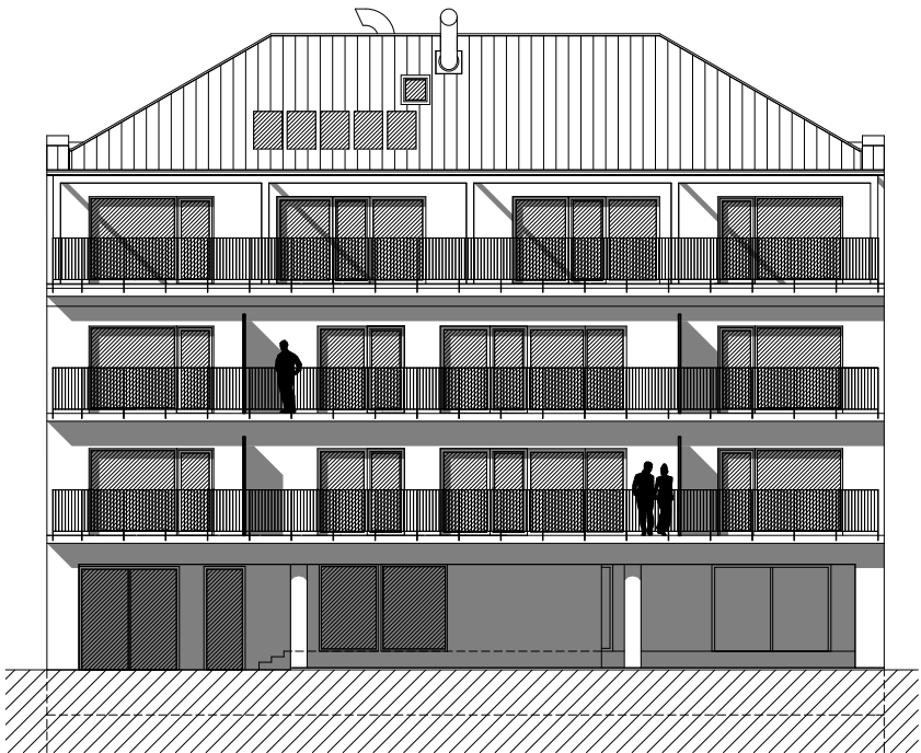
SE Elevation (yard facade)
