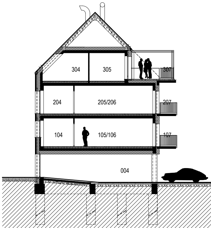
Section BB
