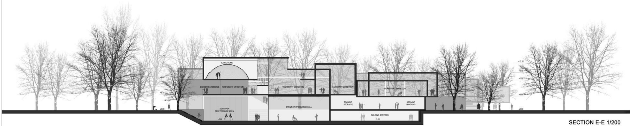
SECTION E-E 1/200
