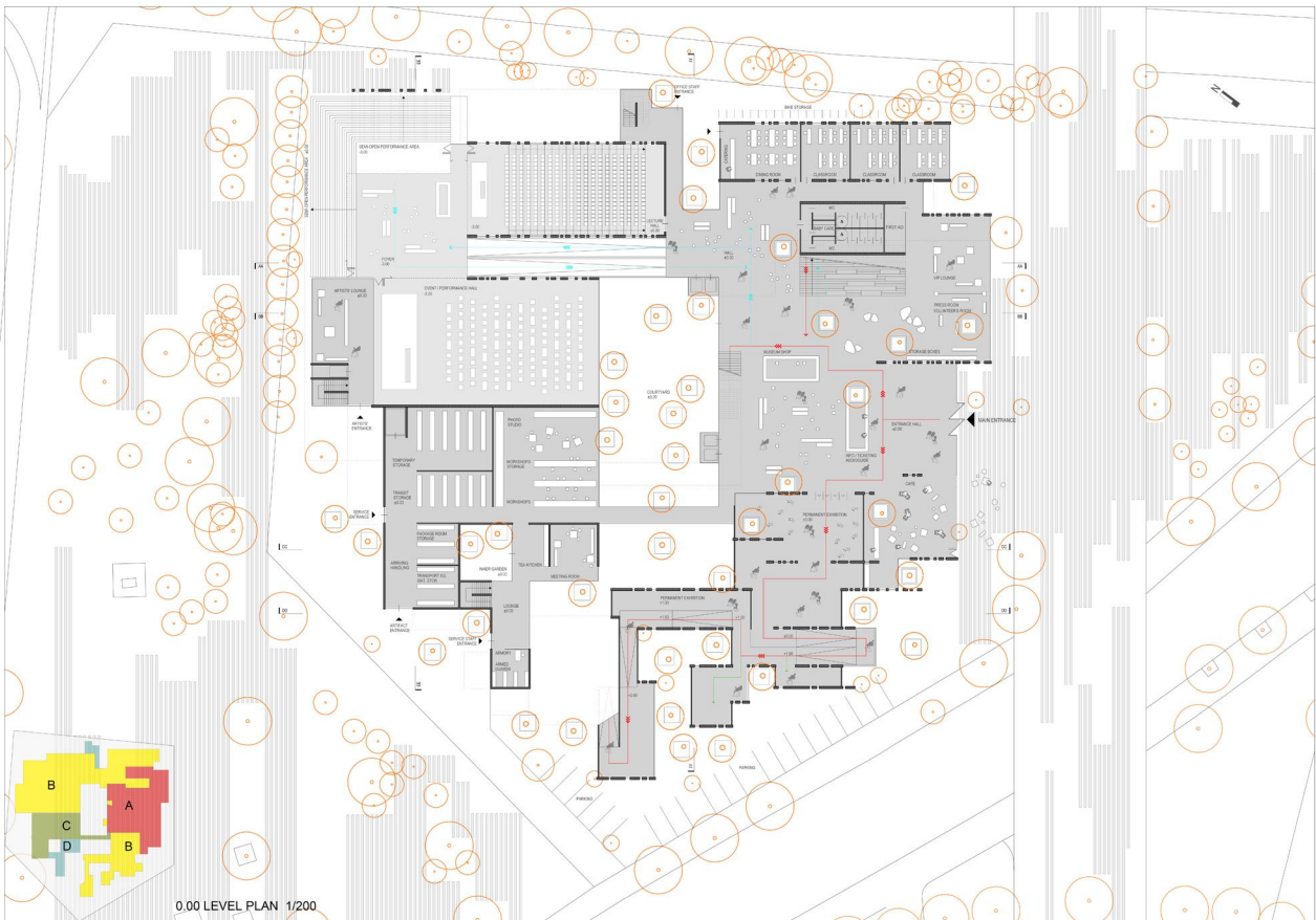
0.00 LEVEL PLAN 1/200
