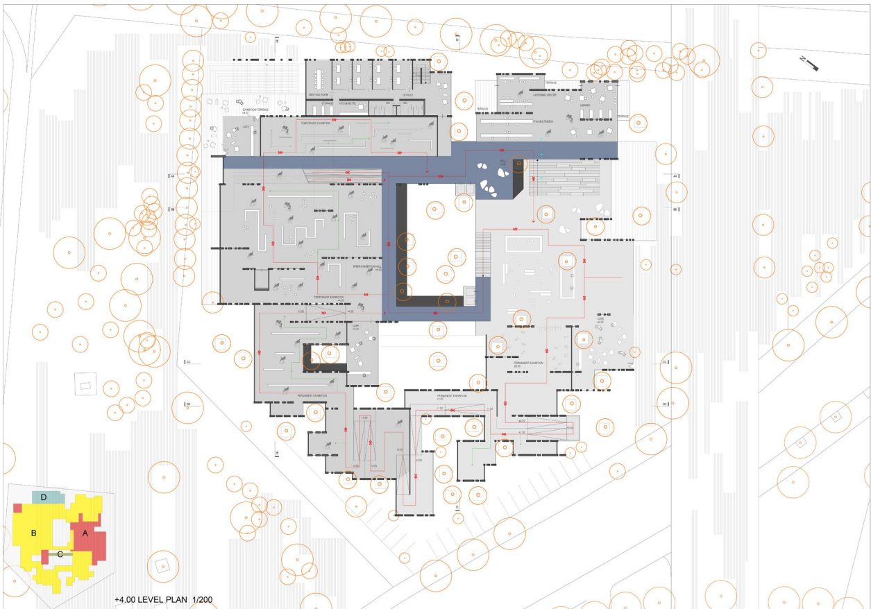
+4.00 LEVEL PLAN 1/200
